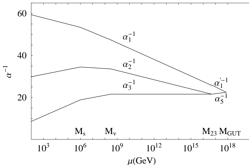
Figure 3: The one-loop gauge coupling unification for M_S = 10^6 GeV and M_V = 3 \times 10^8 GeV.
