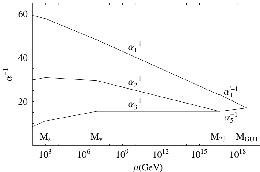
Figure 1: The one-loop gauge coupling unification for M_S = 10^3 GeV and M_V = 10^7 GeV.
