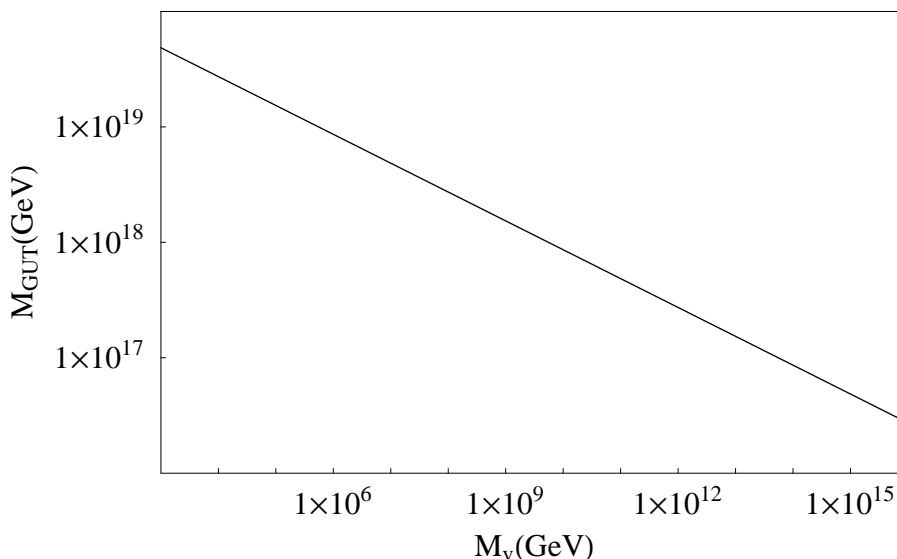
Figure 2: The GUT scale M_{\text{GUT}} versus M_V for M_S = 10^3 GeV, and M_V from 10^3 GeV to 10^{16} GeV.
